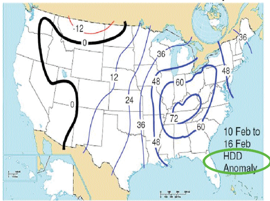
Estimated 10-16 Feb 2006 Gross HDD anomaly
